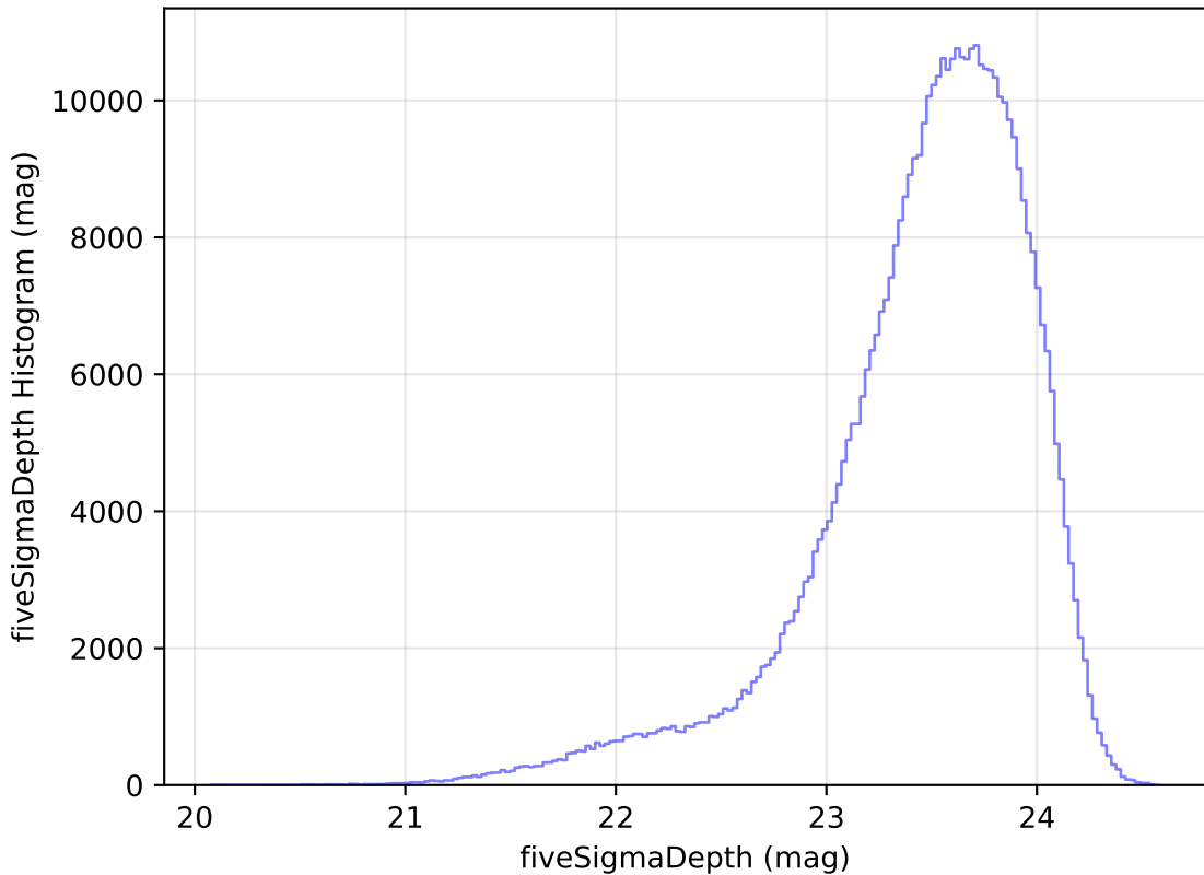
too_elab_r16_d2_gz_v3.4_10yrs All sky i band: fiveSigmaDepth Histogram
