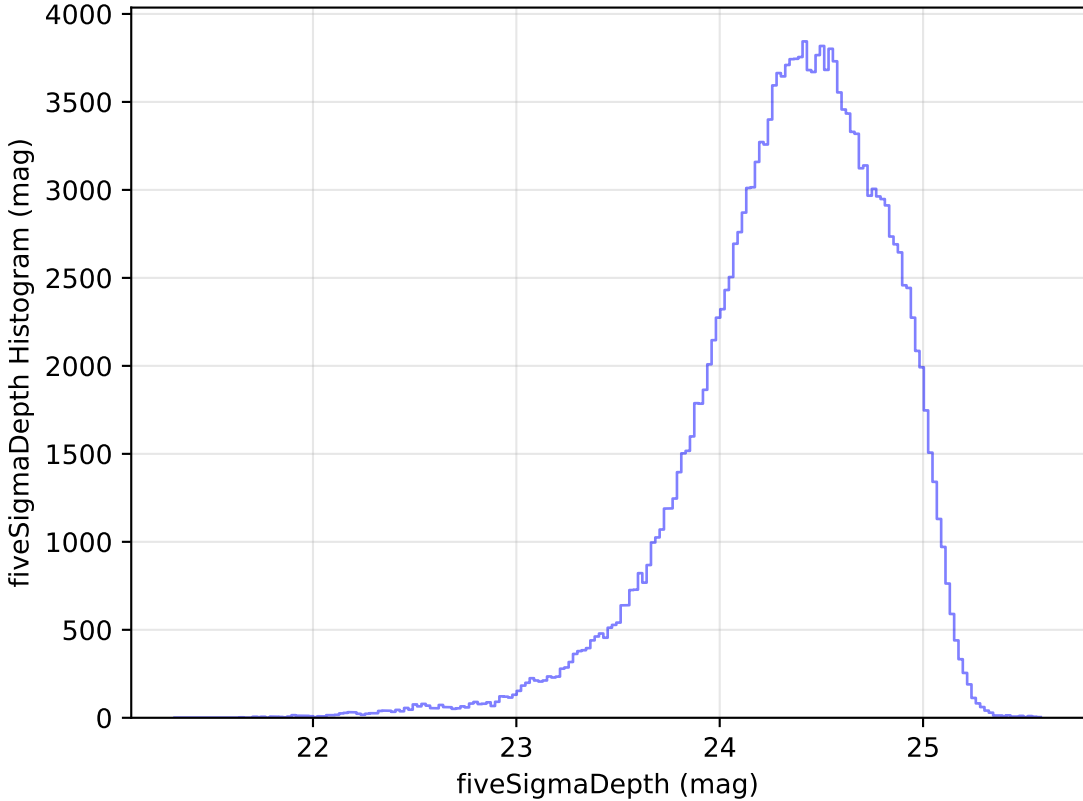
too_elab_r16_d2_gz_v3.4_10yrs All sky g band: fiveSigmaDepth Histogram
