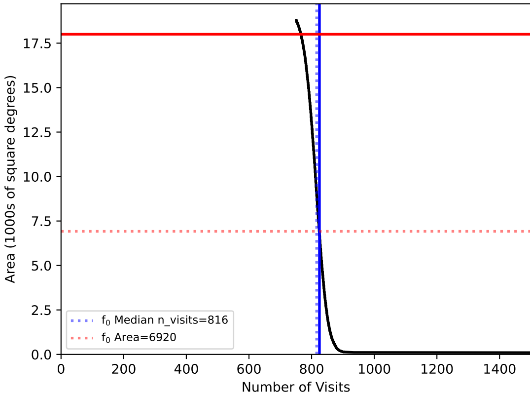
too_elab_r16_d2_gz_v3.4_10yrs WFD: f0
