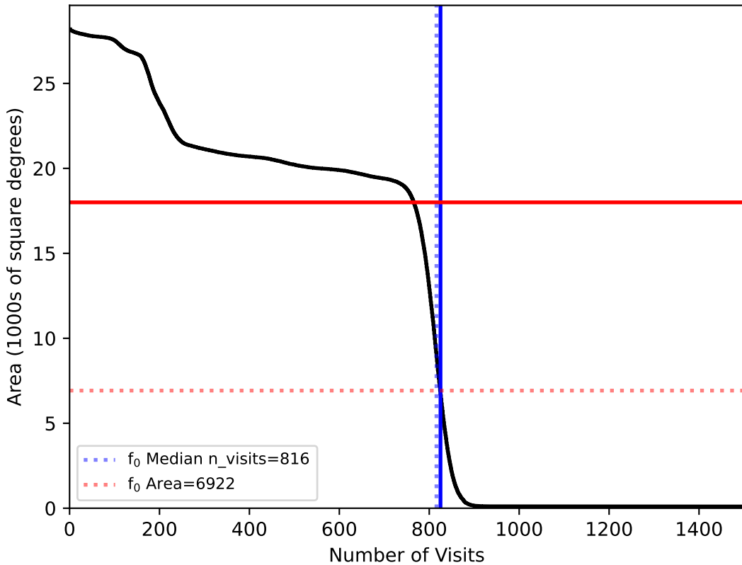
too_elab_r16_d2_gz_v3.4_10yrs All sky: fO
