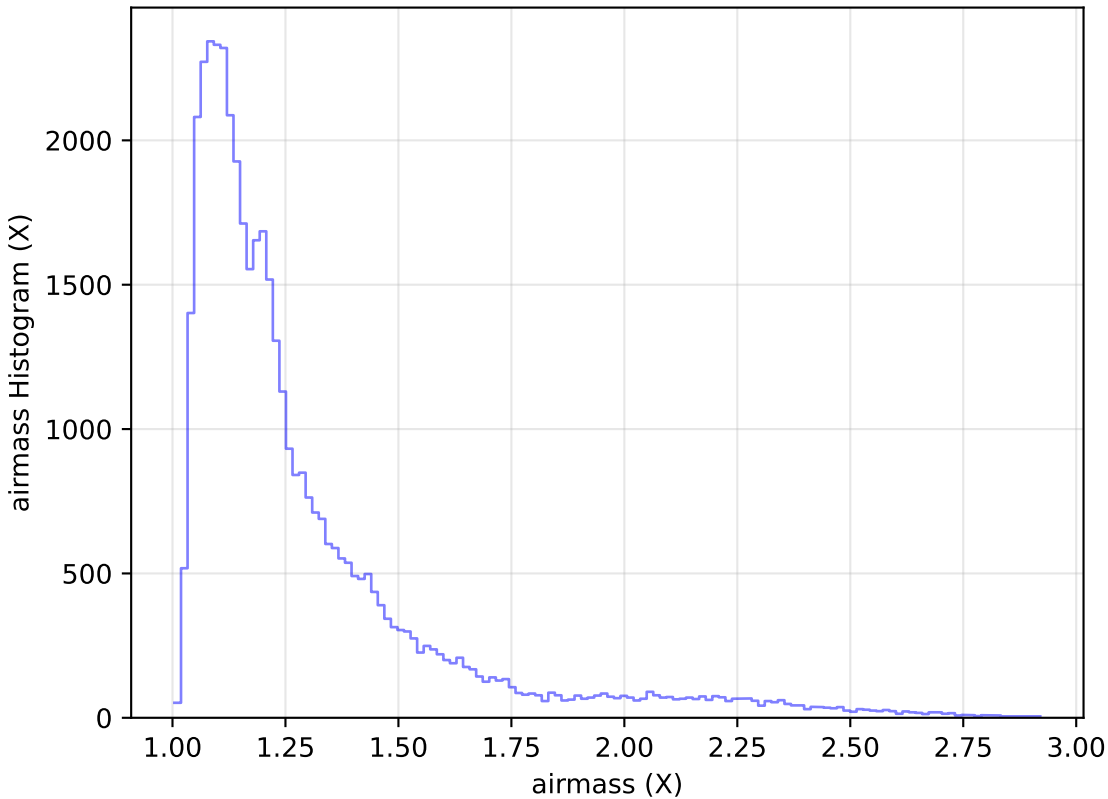
too_elab_r16_d2_gz_v3.4_10yrs Yr 1 z band: airmass Histogram
