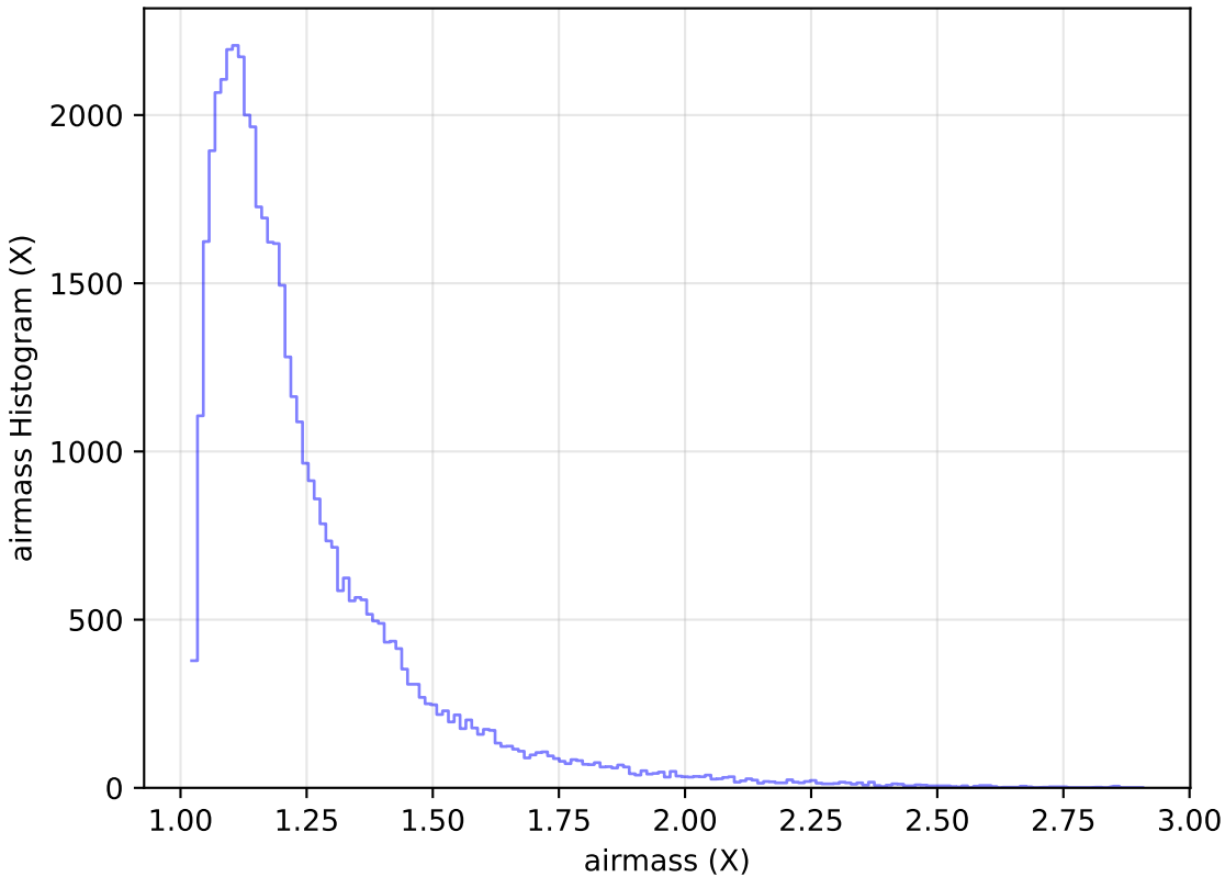
too_elab_r16_d2_gz_v3.4_10yrs Yr 1 y band: airmass Histogram
