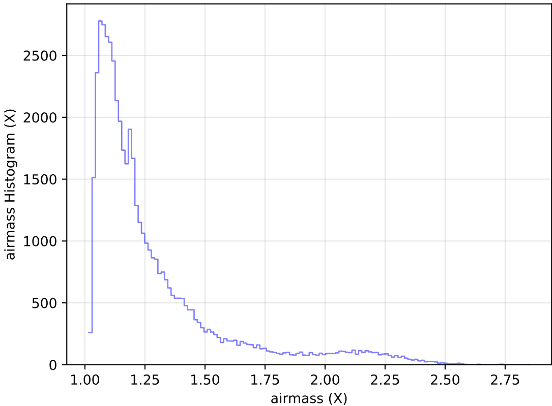
too_elab_r16_d2_gz_v3.4_10yrs Yr 1 r band: airmass Histogram
