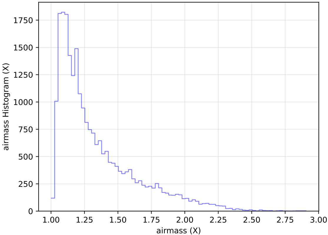
too_elab_r16_d2_gz_v3.4_10yrs Yr 1 g band: airmass Histogram
