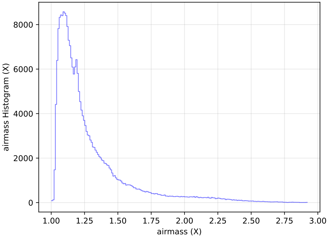
too_elab_r16_d2_gz_v3.4_10yrs Yr 1 all bands: airmass Histogram
