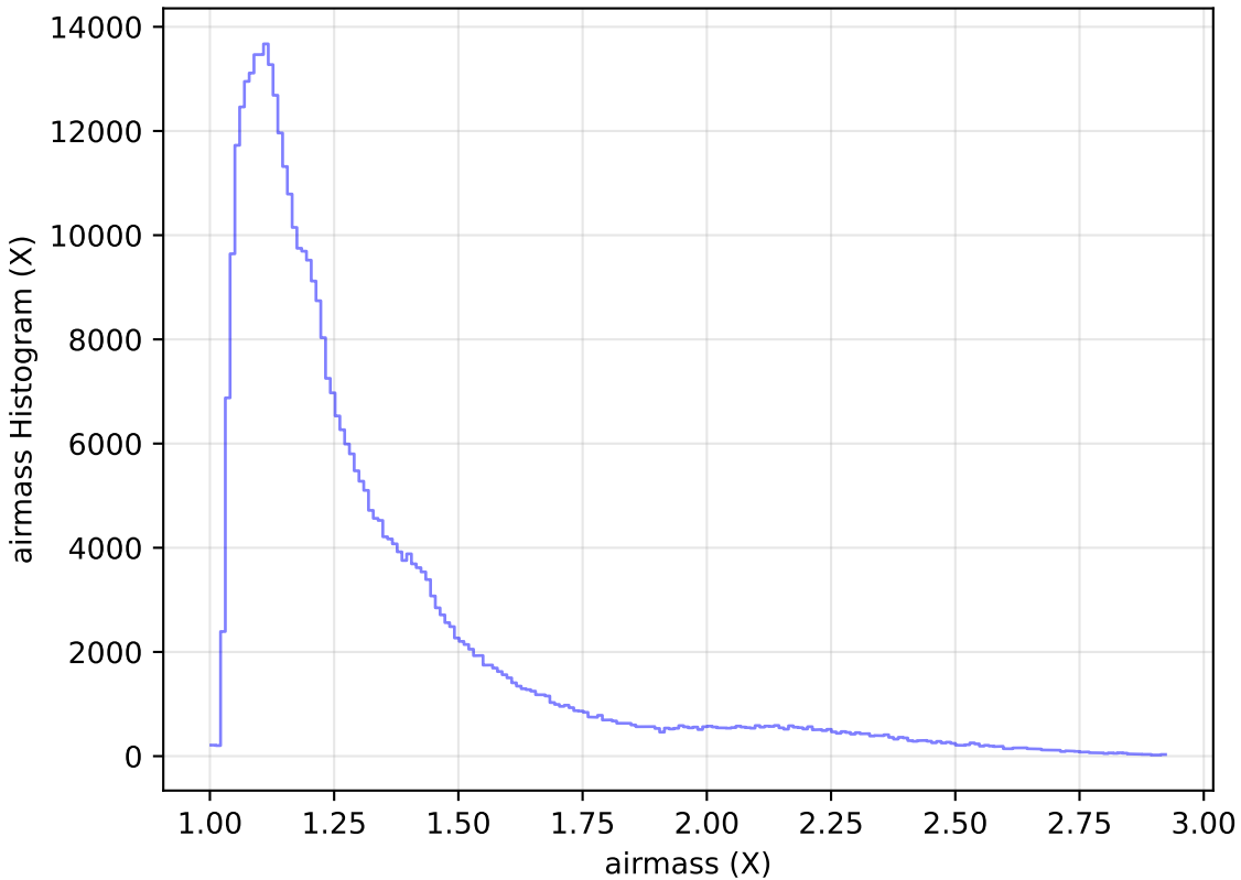
too_elab_r16_d2_gz_v3.4_10yrs WFD z band: airmass Histogram
