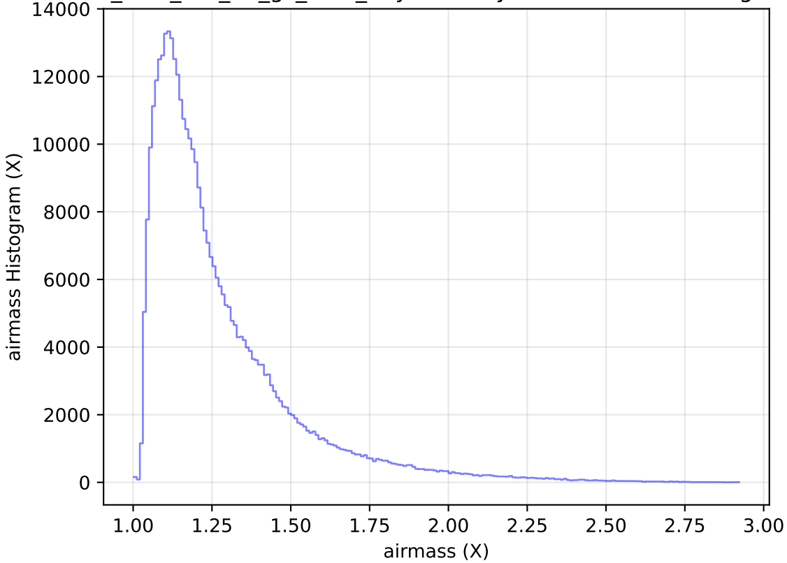
too_elab_r16_d2_gz_v3.4_10yrs WFD y band: airmass Histogram
