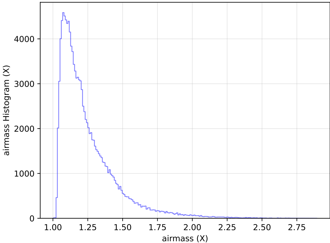
too_elab_r16_d2_gz_v3.4_10yrs WFD u band: airmass Histogram
