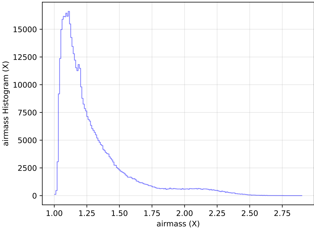
too_elab_r16_d2_gz_v3.4_10yrs WFD r band: airmass Histogram
