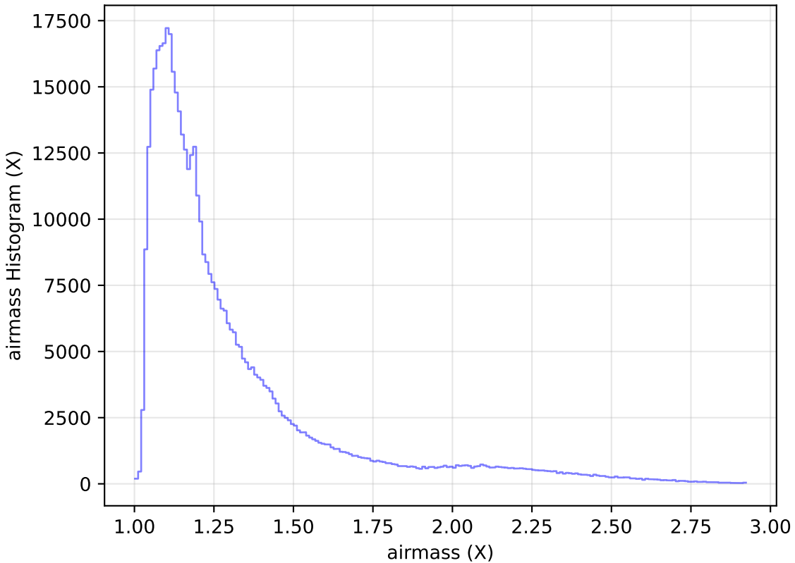
too_elab_r16_d2_gz_v3.4_10yrs WFD i band: airmass Histogram
