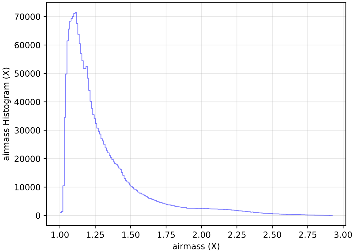
too_elab_r16_d2_gz_v3.4_10yrs WFD all bands: airmass Histogram
