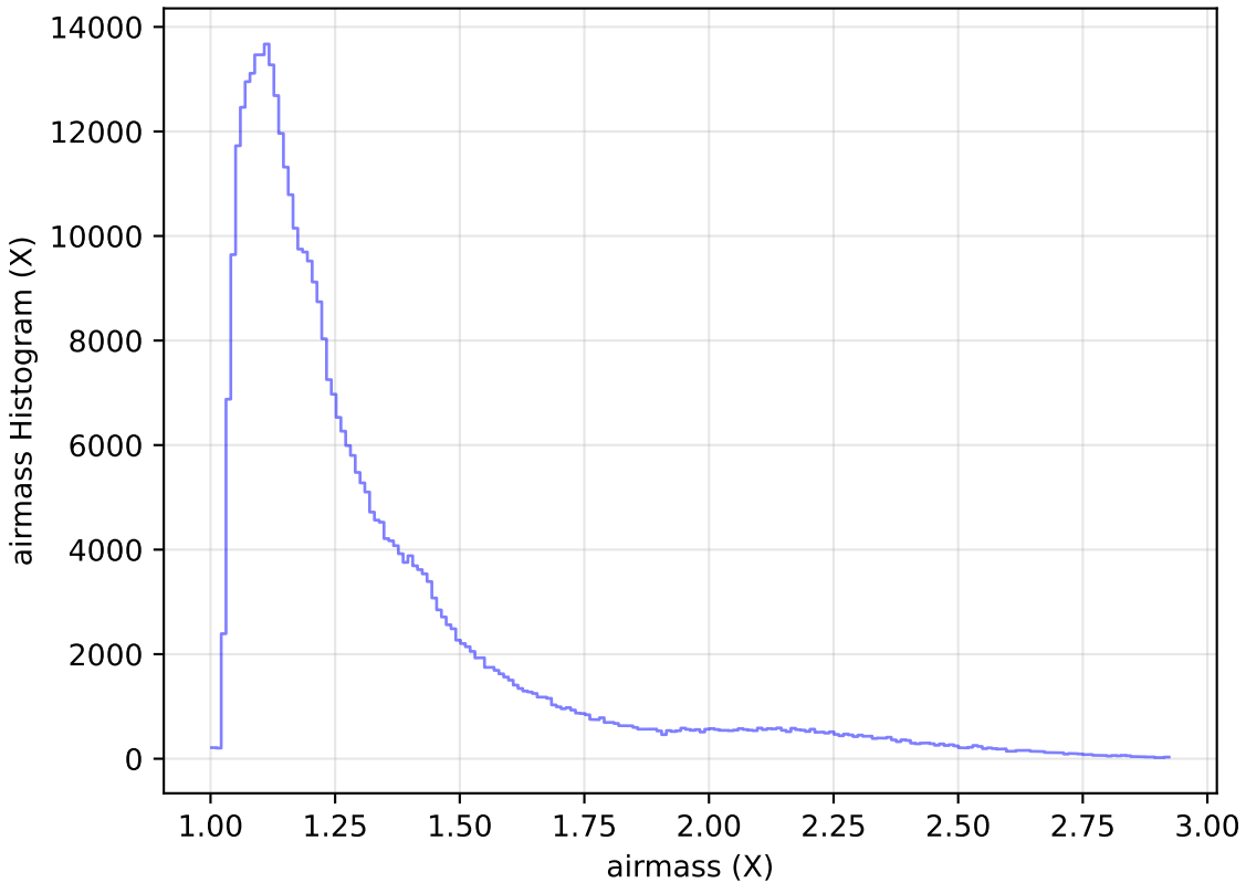
too_elab_r16_d2_gz_v3.4_10yrs All sky z band: airmass Histogram
