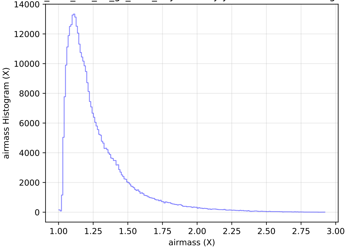
too_elab_r16_d2_gz_v3.4_10yrs All sky y band: airmass Histogram
