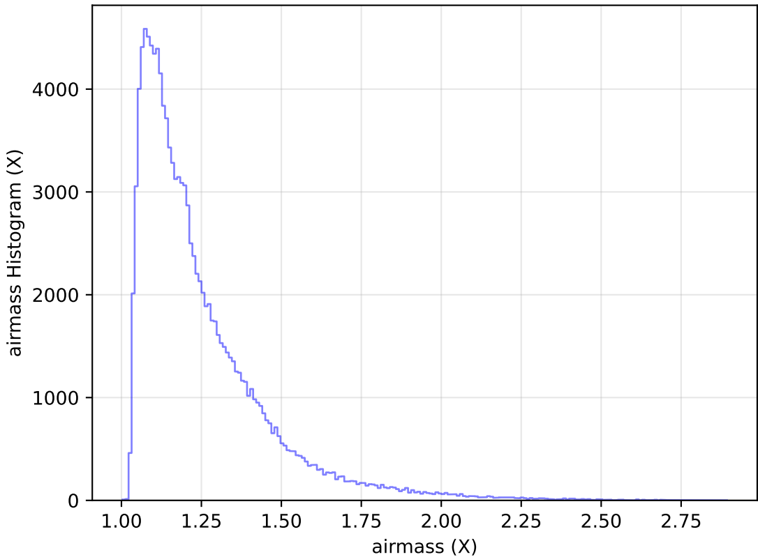
too_elab_r16_d2_gz_v3.4_10yrs All sky u band: airmass Histogram
