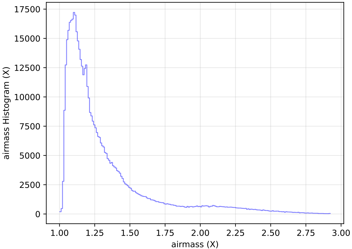
too_elab_r16_d2_gz_v3.4_10yrs All sky i band: airmass Histogram
