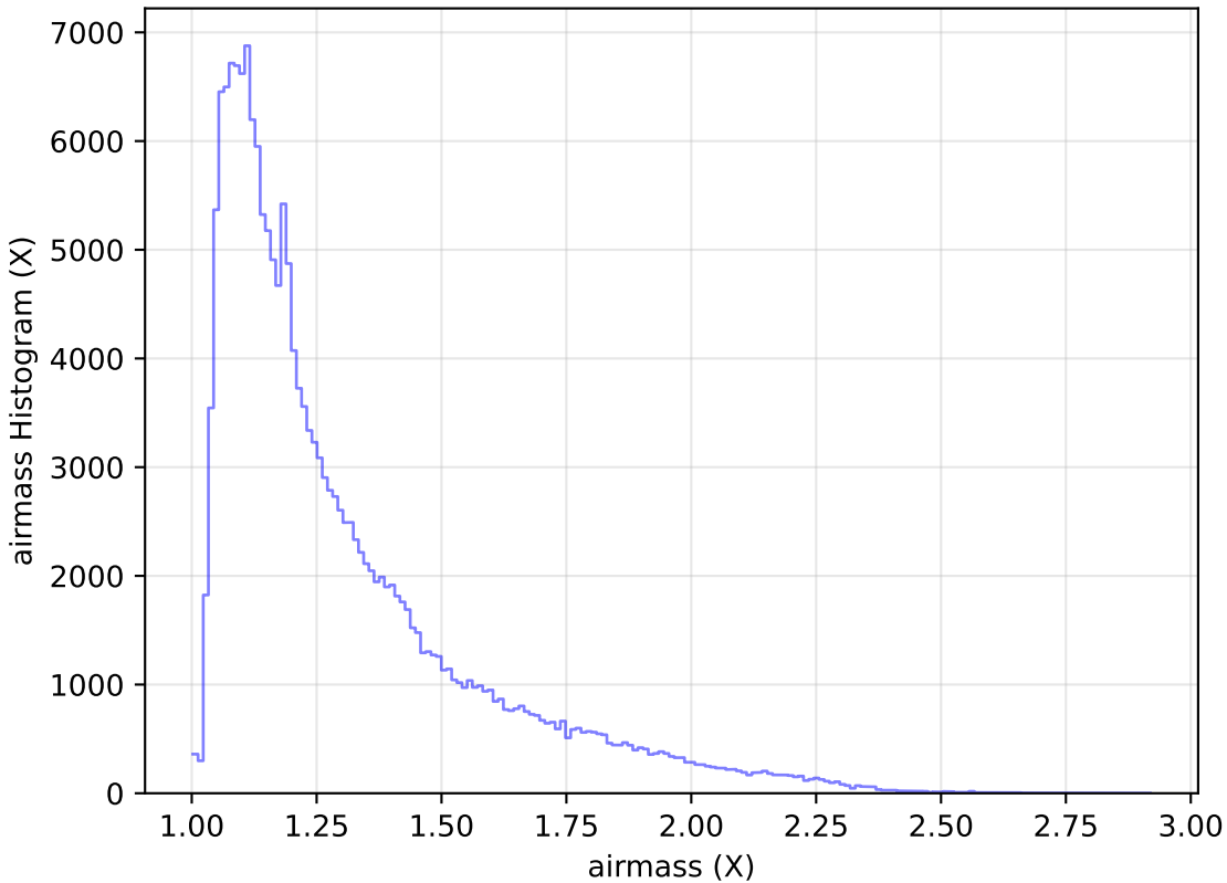
too_elab_r16_d2_gz_v3.4_10yrs All sky g band: airmass Histogram
