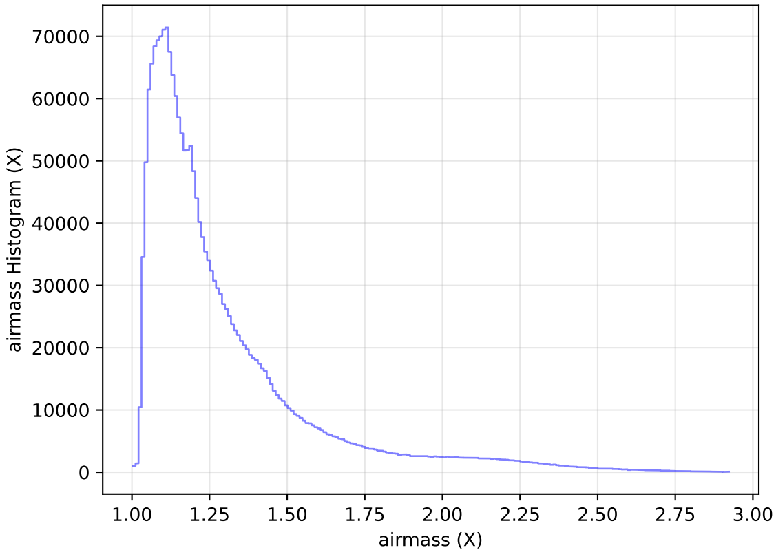
too_elab_r16_d2_gz_v3.4_10yrs All sky all bands: airmass Histogram
