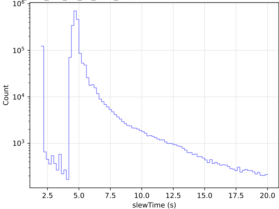
too_elab_r16_d2_gz_v3.4_10yrs All visits: Zoom Slew Time Histogram
