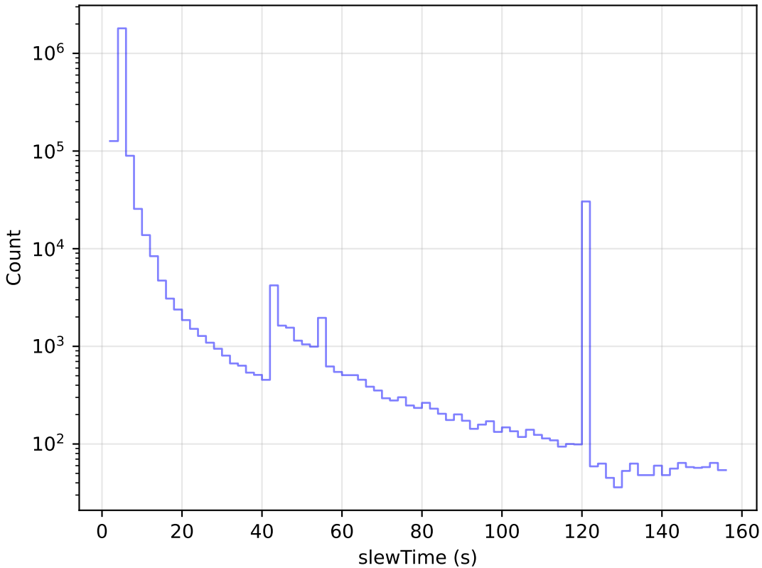
too_elab_r16_d2_gz_v3.4_10yrs All visits: Slew Time Histogram
