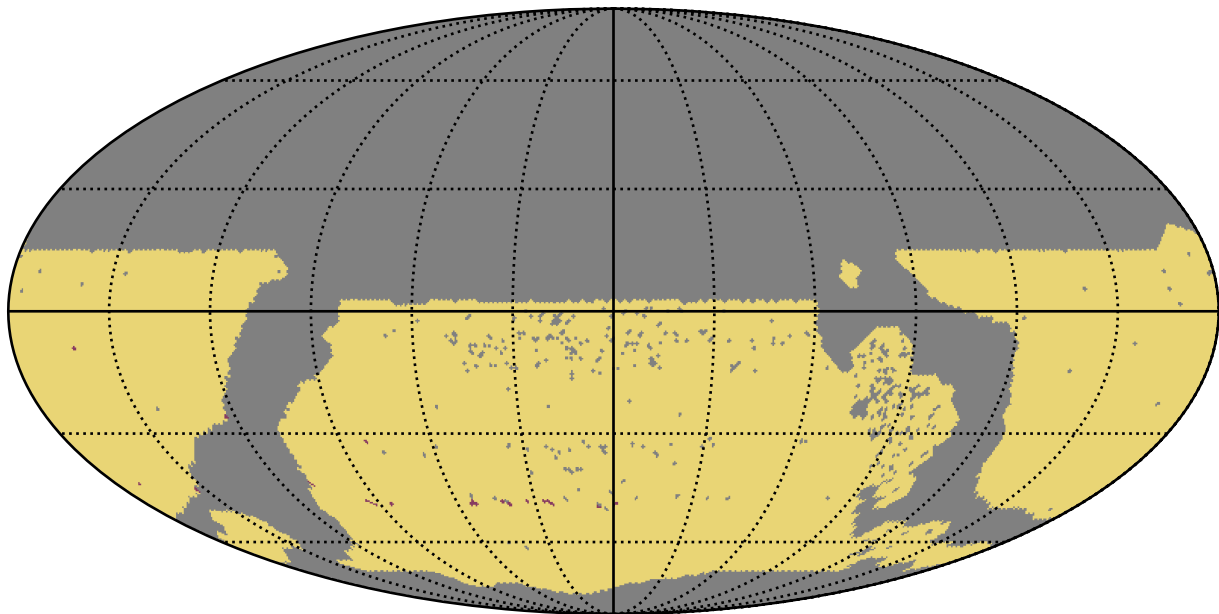
too_elab_r16_d2_gz_v3.4_10yrs WFD: RapidRevisits
