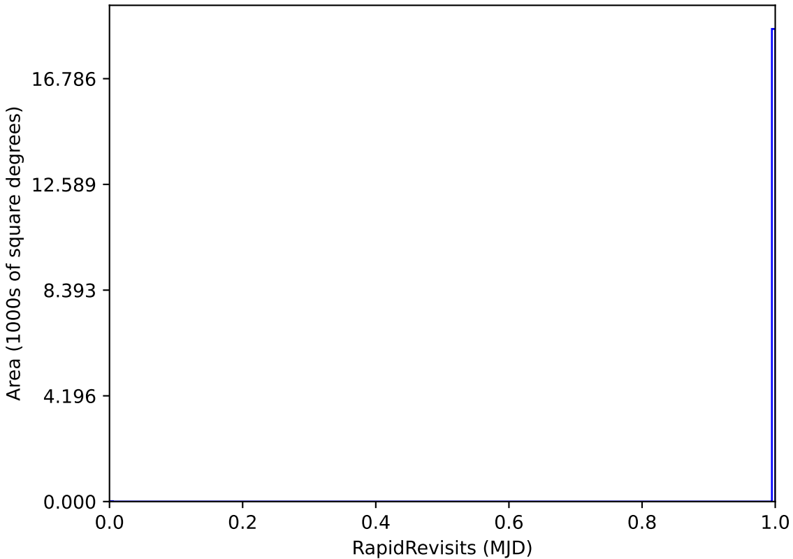
too_elab_r16_d2_gz_v3.4_10yrs WFD: RapidRevisits
