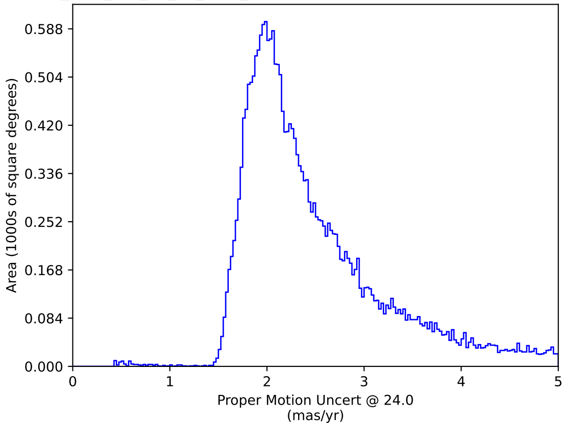
too_elab_r16_d2_gz_v3.4_10yrs All sky: Proper Motion Uncert @ 24.0
