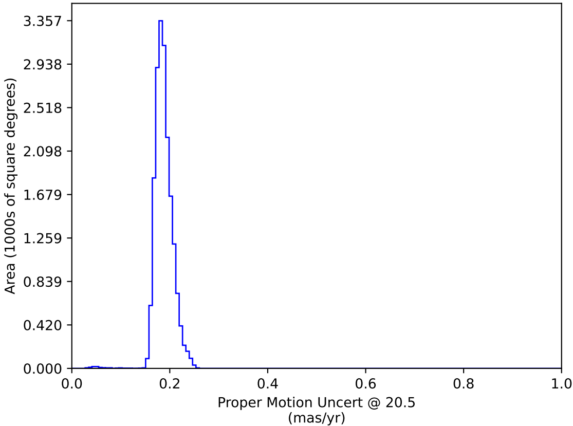
too_elab_r16_d2_gz_v3.4_10yrs WFD: Proper Motion Uncert @ 20.5
