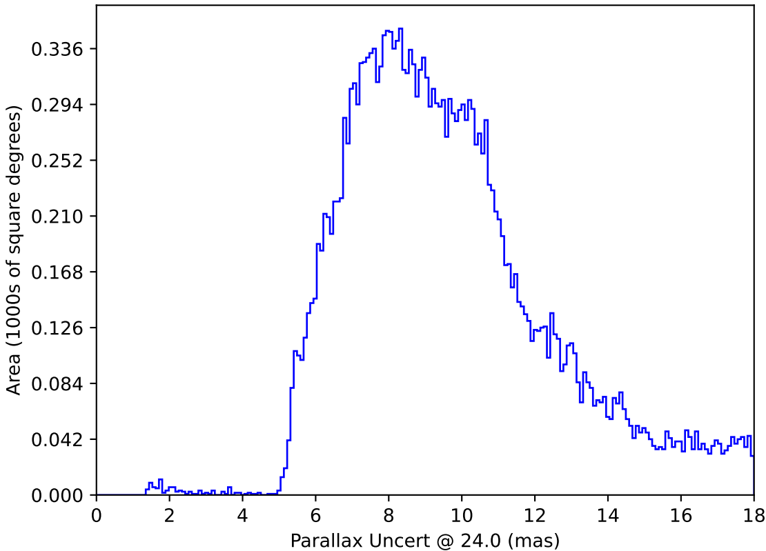
too_elab_r16_d2_gz_v3.4_10yrs All sky: Parallax Uncert @ 24.0
