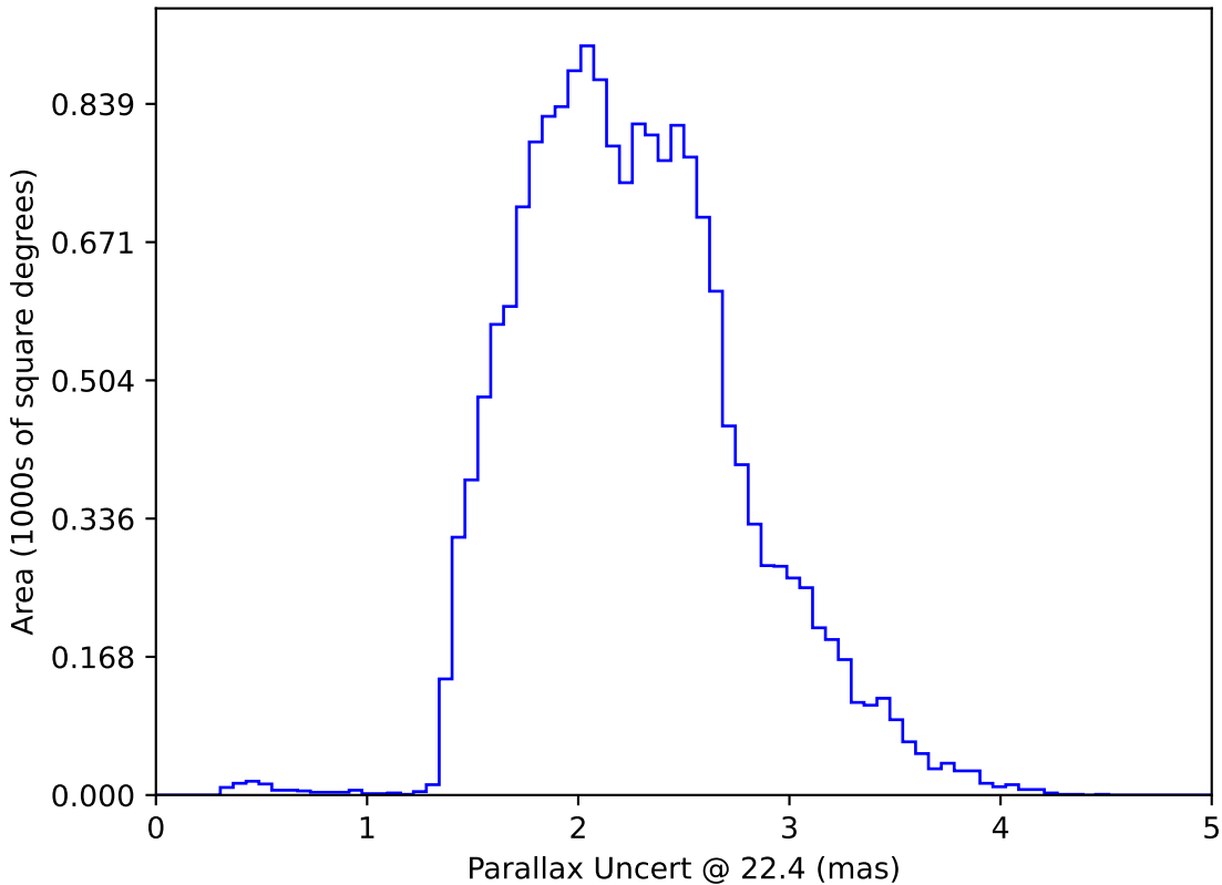
too_elab_r16_d2_gz_v3.4_10yrs WFD: Parallax Uncert @ 22.4
