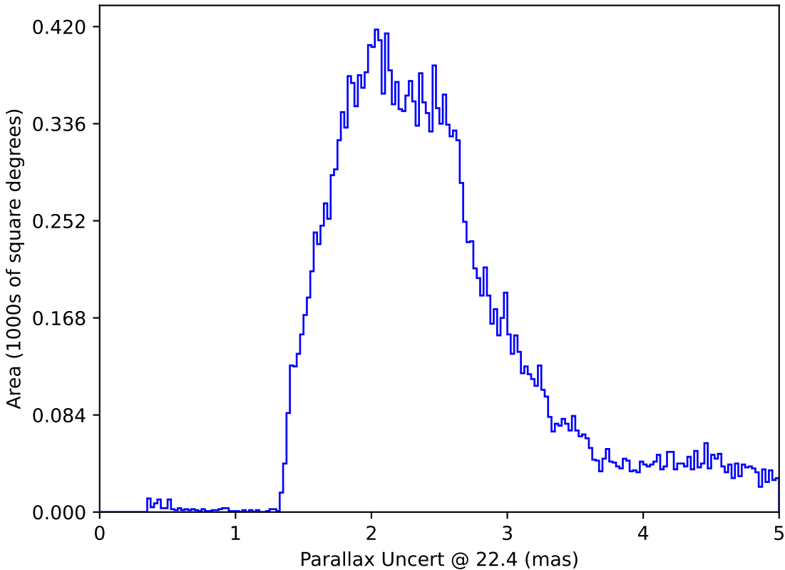
too_elab_r16_d2_gz_v3.4_10yrs All sky: Parallax Uncert @ 22.4
