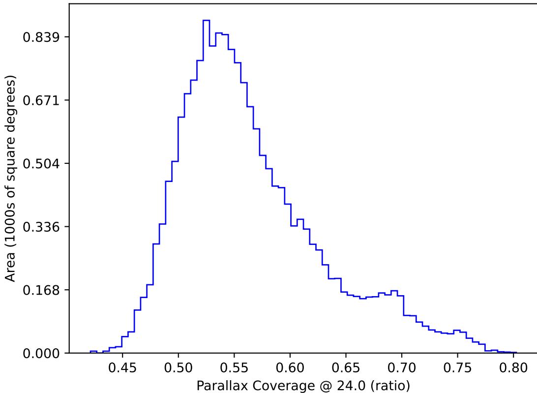
too_elab_r16_d2_gz_v3.4_10yrs WFD: Parallax Coverage @ 24.0
