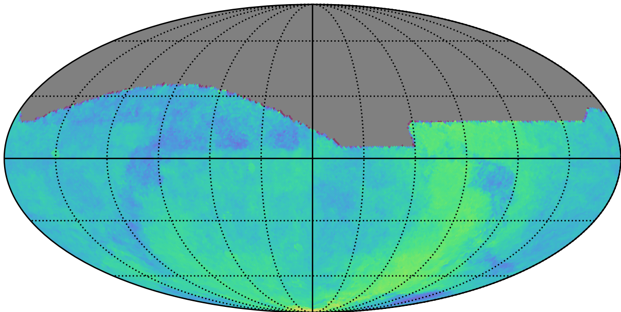
too_elab_r16_d2_gz_v3.4_10yrs All sky: Parallax Coverage @ 24.0
