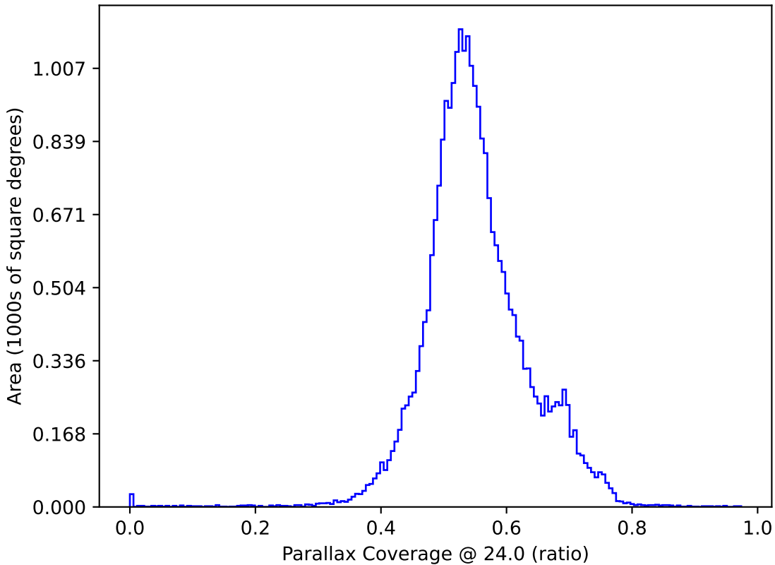
too_elab_r16_d2_gz_v3.4_10yrs All sky: Parallax Coverage @ 24.0
