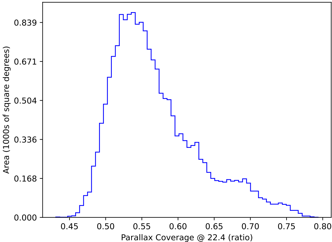
too_elab_r16_d2_gz_v3.4_10yrs WFD: Parallax Coverage @ 22.4
