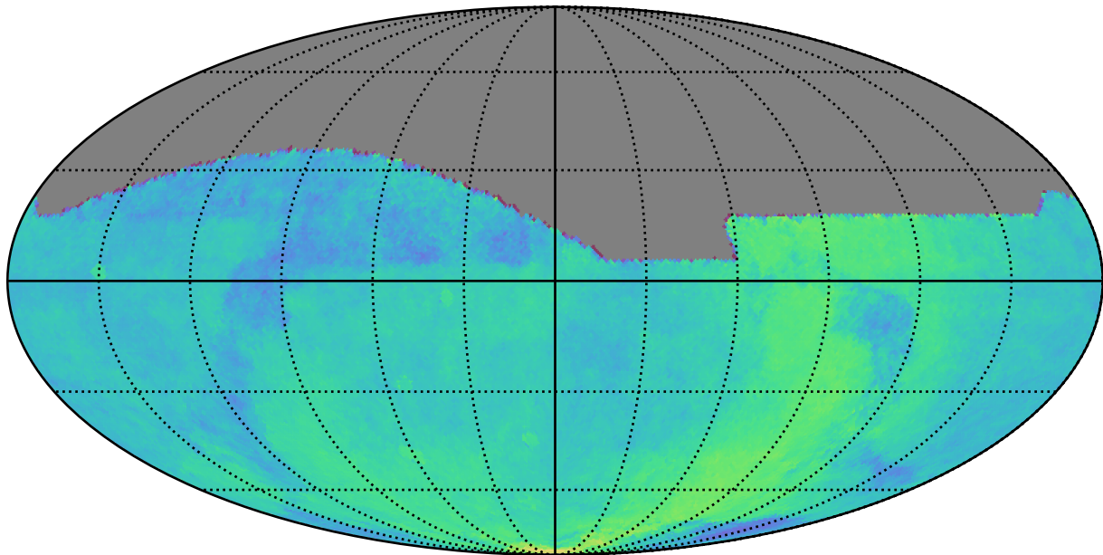
too_elab_r16_d2_gz_v3.4_10yrs All sky: Parallax Coverage @ 22.4
