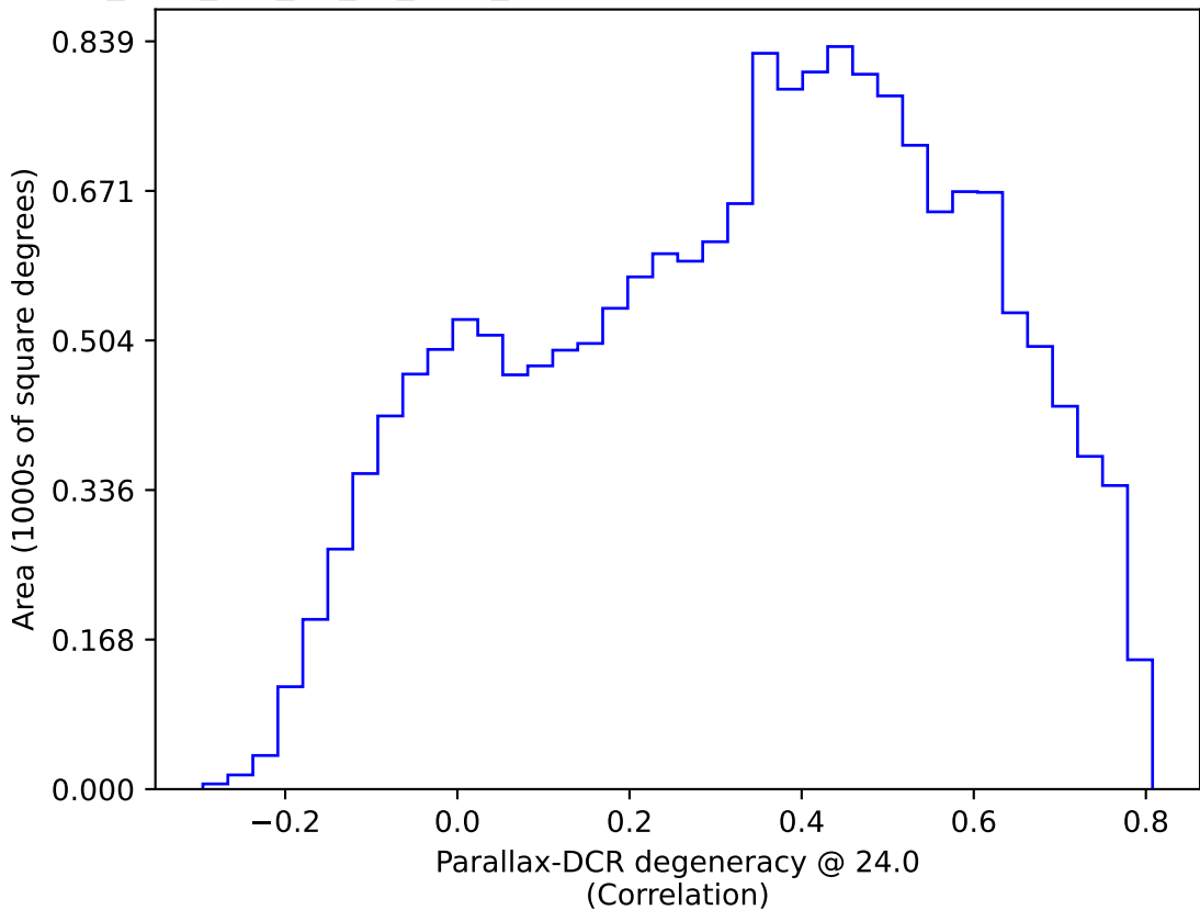
too_elab_r16_d2_gz_v3.4_10yrs WFD: Parallax-DCR degeneracy @ 24.0
