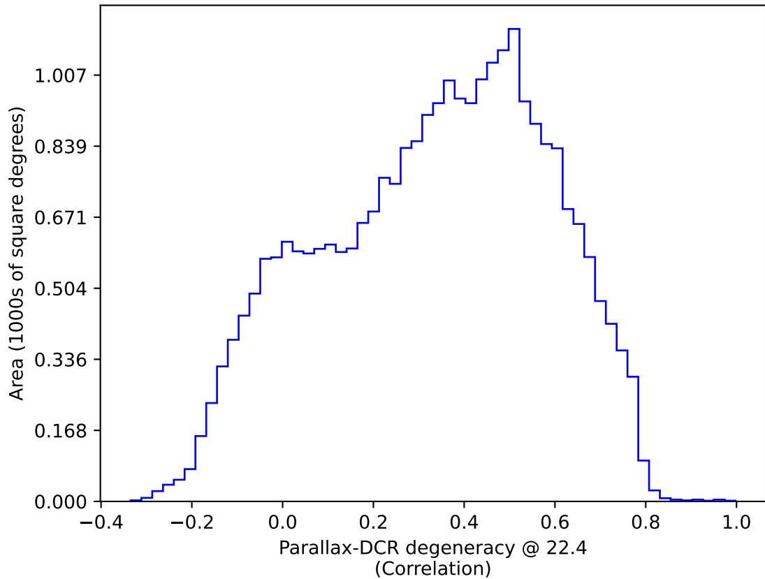
too_elab_r16_d2_gz_v3.4_10yrs All sky: Parallax-DCR degeneracy @ 22.4
