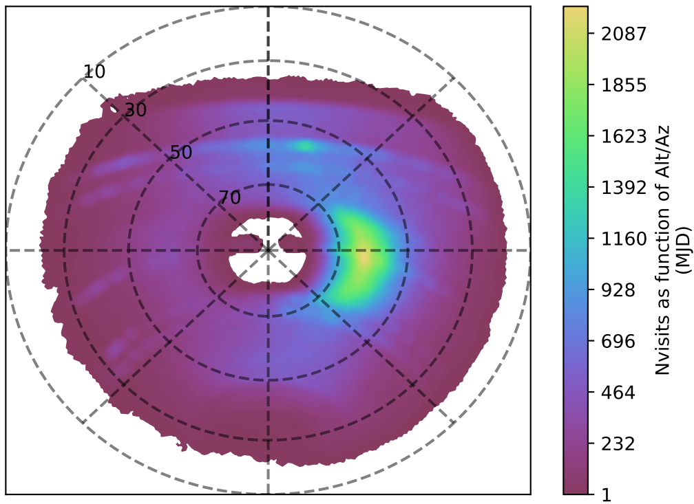
too_elab_r16_d2_gz_v3.4_10yrs y band: Nvisits as function of Alt/Az
