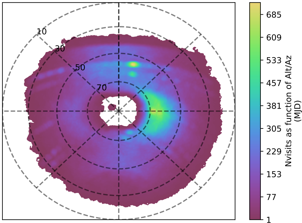
too_elab_r16_d2_gz_v3.4_10yrs u band: Nvisits as function of Alt/Az
