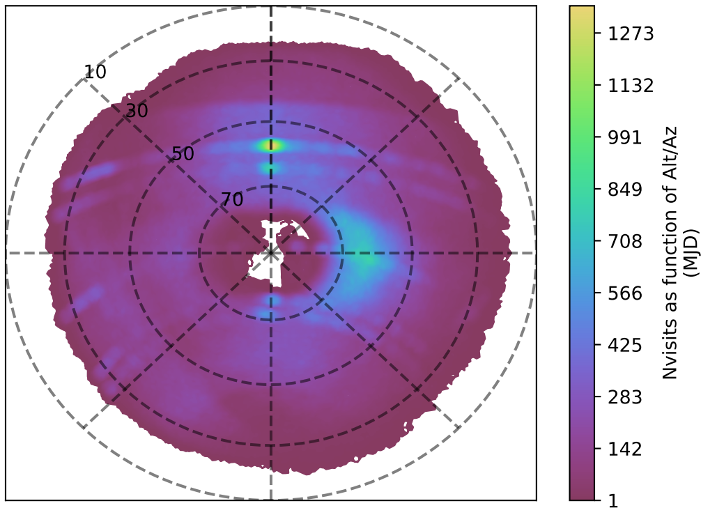
too_elab_r16_d2_gz_v3.4_10yrs g band: Nvisits as function of Alt/Az
