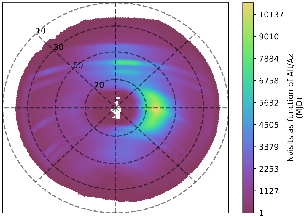
too_elab_r16_d2_gz_v3.4_10yrs all bands: Nvisits as function of Alt/Az
