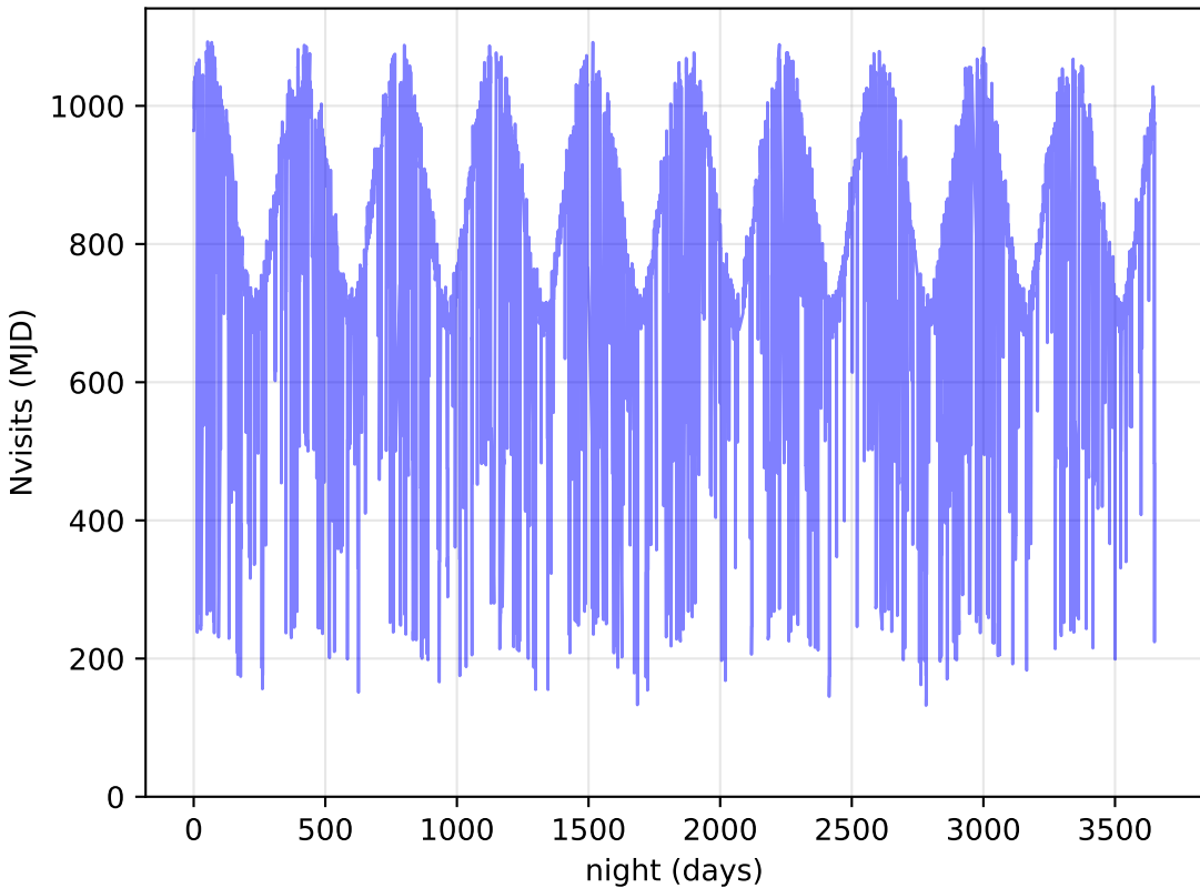
too_elab_r16_d2_gz_v3.4_10yrs All visits: Nvisits
