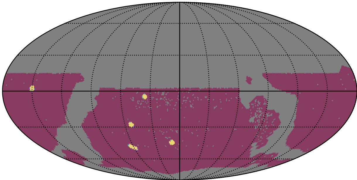
too_elab_r16_d2_gz_v3.4_10yrs WFD: NumberOfQuickRevisits
