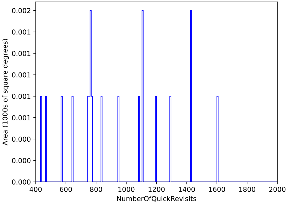
too_elab_r16_d2_gz_v3.4_10yrs WFD: NumberOfQuickRevisits
