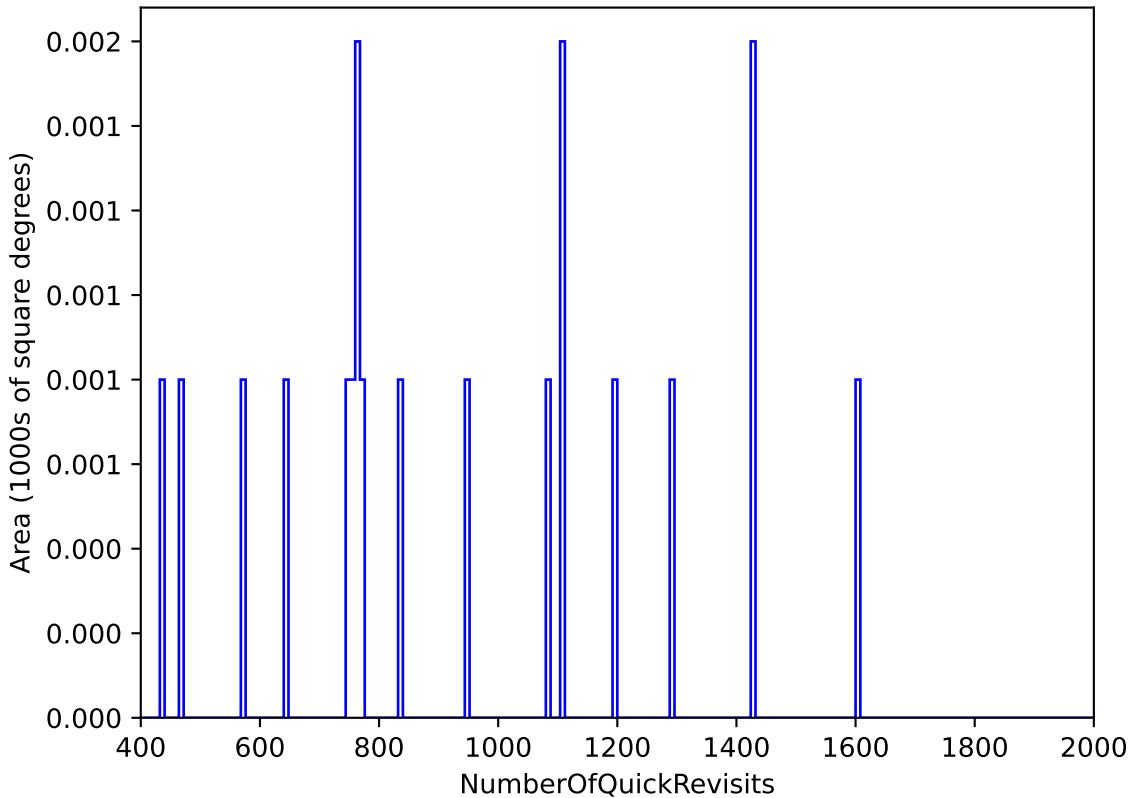
too_elab_r16_d2_gz_v3.4_10yrs All sky: NumberOfQuickRevisits
