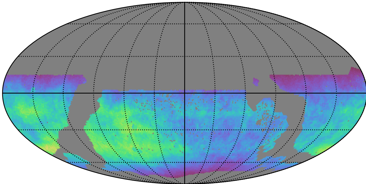
too_elab_r16_d2_gz_v3.4_10yrs WFD z band: Normalized Teff
