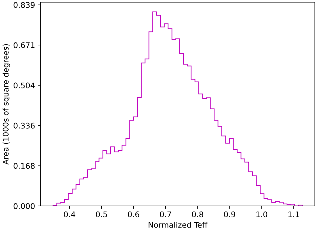
too_elab_r16_d2_gz_v3.4_10yrs WFD z band: Normalized Teff
