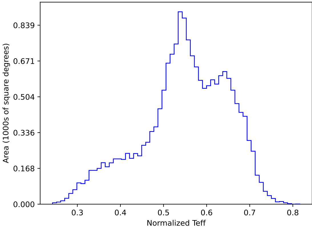
too_elab_r16_d2_gz_v3.4_10yrs WFD y band: Normalized Teff
