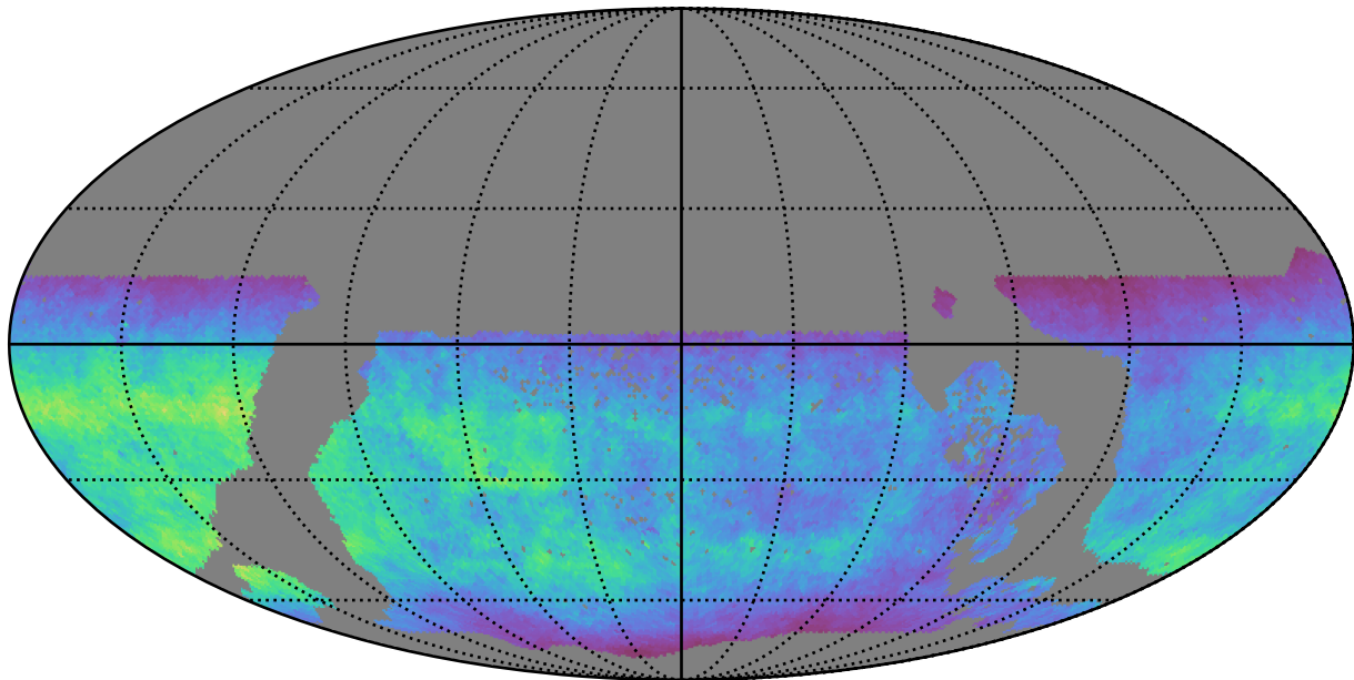
too_elab_r16_d2_gz_v3.4_10yrs WFD u band: Normalized Teff
