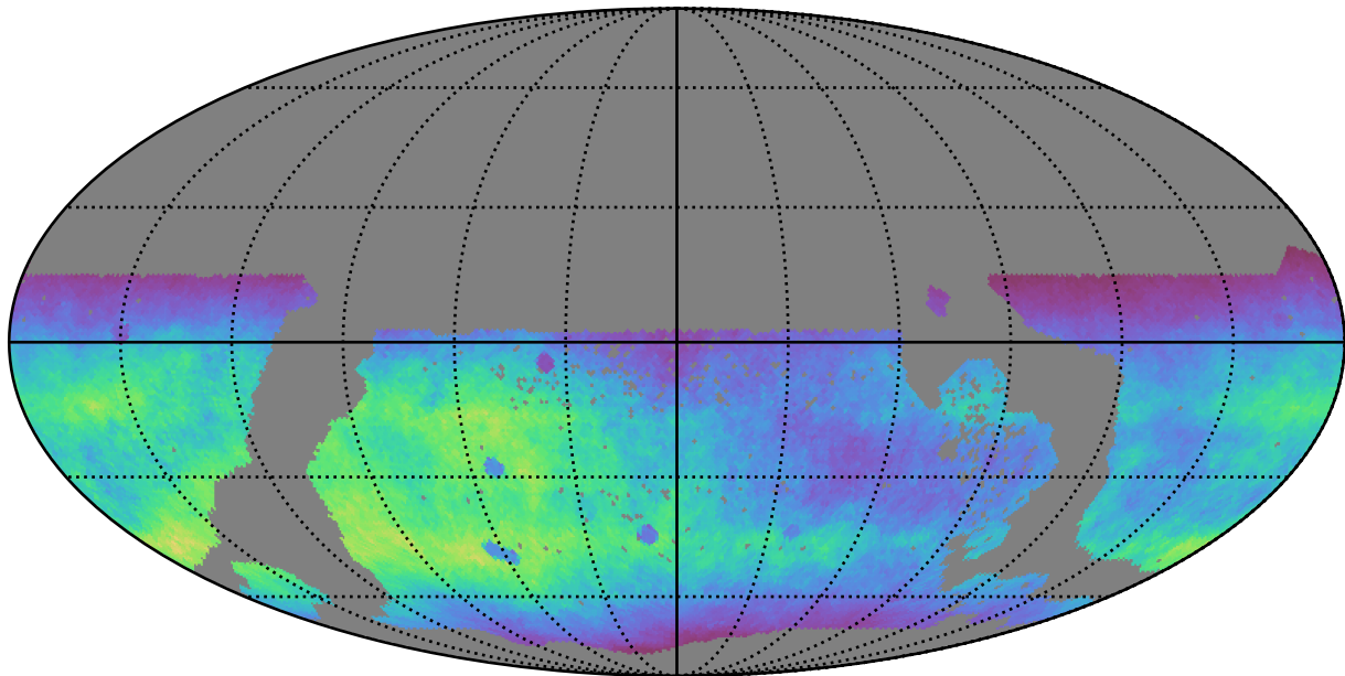
too_elab_r16_d2_gz_v3.4_10yrs WFD r band: Normalized Teff
